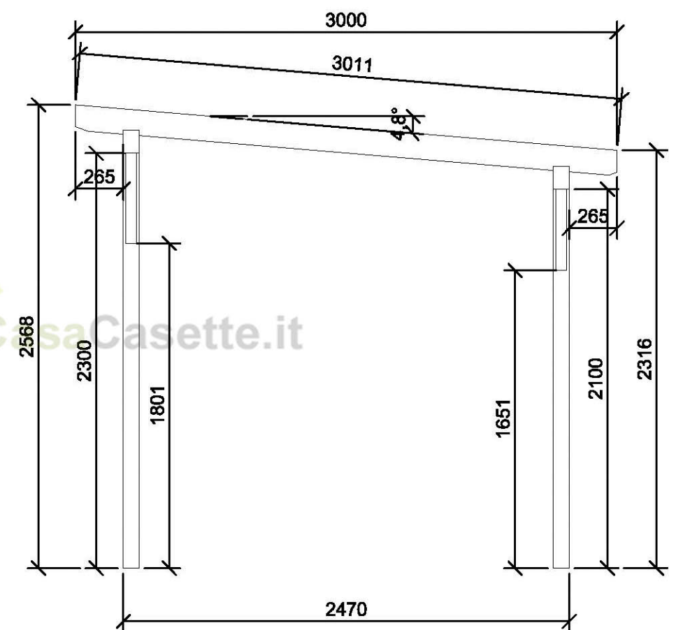
Carport 3x5m 88x88mm
