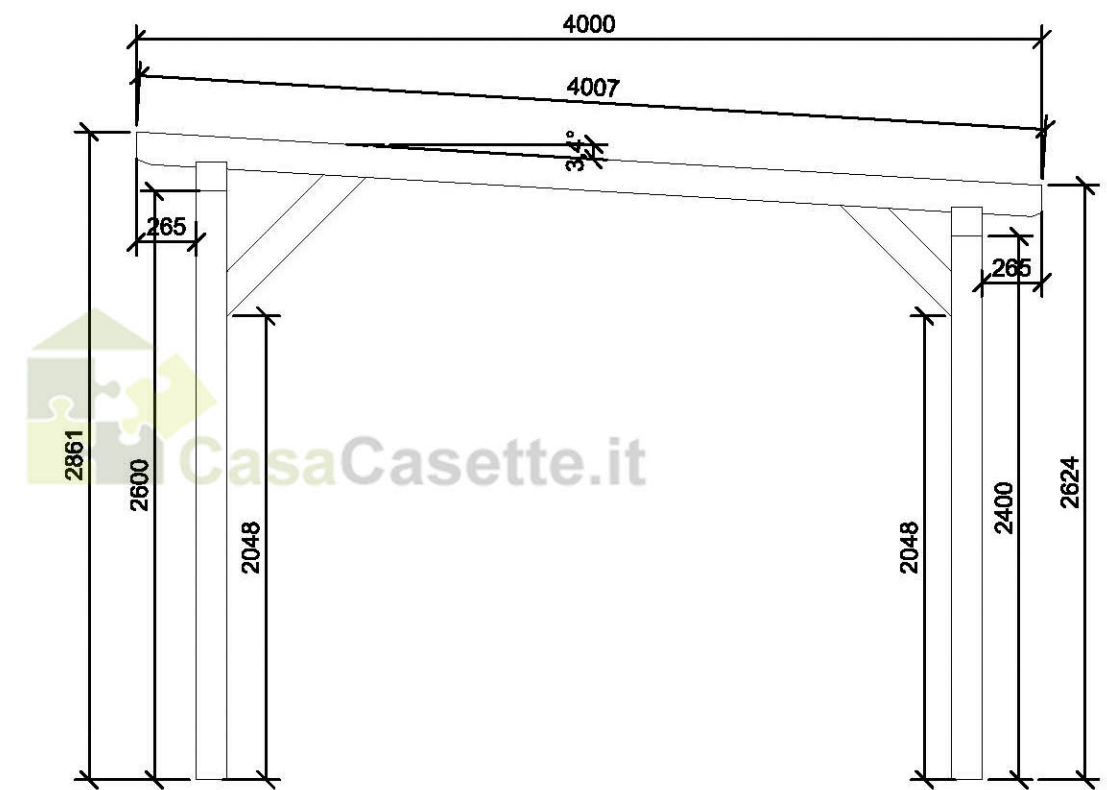
Carport 4x6m 135x135mm
