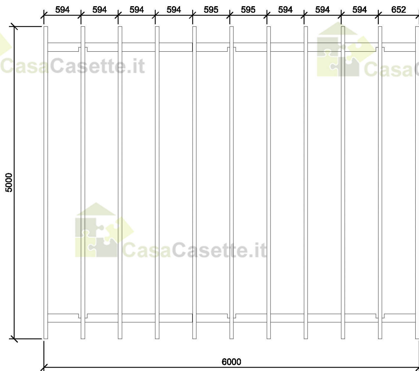
Carport 5x6m 135x135mm
