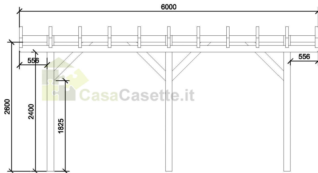
Carport 5x6m 135x135mm
