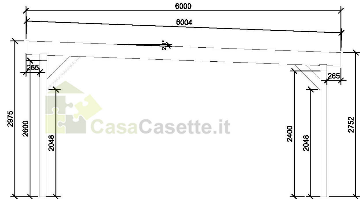
Carport 6x6m 135x135mm
